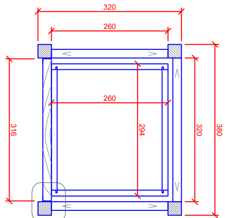
PLAN SECTION A
