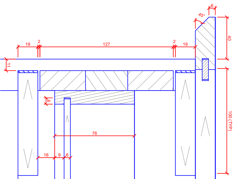
DETAIL #1 SCALE 1:1
