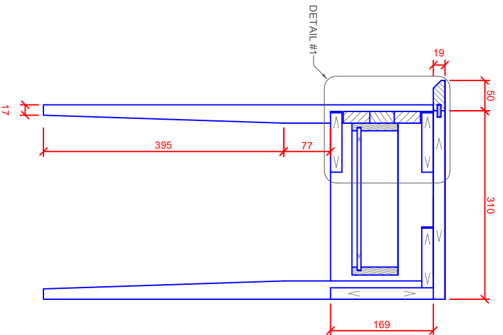
RIGHT SIDE SECTION B
